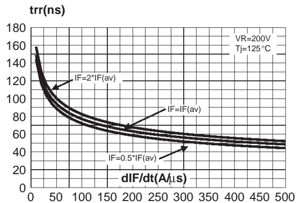
Fig. 5: Reverse recovery time versus di/dt (90% confidence, per diode).
