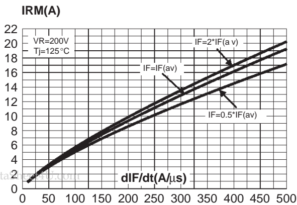
Fig. 4: Peak reverse recovery current versus di/dt (90% confidence, per diode).
